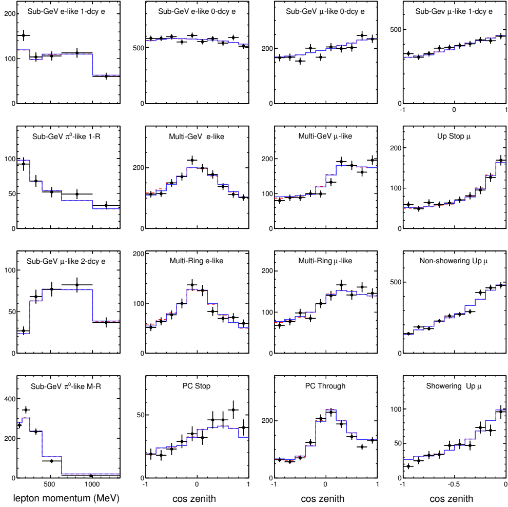
FIG. 10: SK-I+II+III zenith angle and lepton momentum distributions of the event samples used in the analyses. Black dots represent the data with statistical errors, the solid lines are the MC expectation at the best fit from the \theta_{13} analysis, and dashed lines show the expectation at the best fit atmospheric variables but with \theta_{13} at the Chooz limit.
