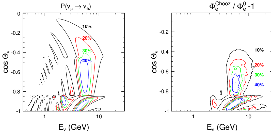
FIG. 2: The three flavor oscillation probability \nu_\mu \leftrightarrow \nu_e for \theta_{13} at the Chooz limit for neutrinos under the normal hierarchy in the one mass scale dominant framework is shown at left. In the right panel the \nu_e flux ratio \Phi_e^{\text{Chooz}}/\Phi_e^0 - 1 for oscillations with \theta_{13} at the Chooz limit relative to those at \theta_{13} = 0 . Large matter-induced resonances between 2-10 GeV appear for upward going neutrinos traversing the core ( \cos\Theta_\nu < -0.84 ) and mantle regions ( -0.84 < \cos\Theta_\nu < -0.45 ). Atmospheric mixing is assumed at \Delta m_{23}^2 = 2.1 \times 10^{-3} \text{ eV}^2 and \sin^2\theta_{23} = 0.5 .
