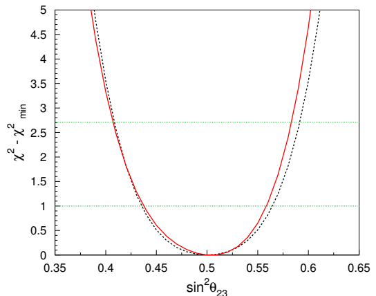
FIG. 5: \chi^2 - \chi_{min}^2 distribution as a function of \sin^2\theta_{23} for oscillations without the 1-2 parameters (dotted line) and with the 1-2 parameters (solid line). For each \sin^2\theta_{23} point, \Delta m_{23}^2 is chosen so that \chi^2 is minimized. The horizontal line corresponds to the 68%(90%) confidence level which is located at \chi_{min}^2 + 1.0(2.7) .
