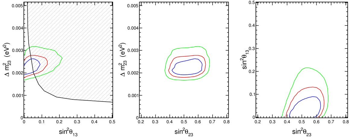
FIG. 8: Inverted hierarchy contours for the SK-I+II+III data set. The 68%, 90%, and 99% allowed region appear in blue, red, and green respectively. The shaded region in the first panel shows the Chooz 90% exclusion region.
