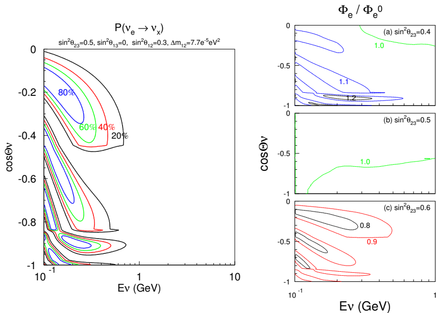
FIG. 1: The left side of the figure shows the calculated \nu_e transition probability P_{ex} for atmospheric neutrinos with an energy E_\nu and neutrino zenith angle, \cos\Theta_\nu , using \Delta m_{12}^2 = 7.7 \times 10^{-5} eV^2 \sin^2\theta_{12} = 0.3 [27], \sin^2\theta_{23} = 0.5, \sin^2\theta_{13} = 0.0 and \Delta m_{23}^2 = 2.1 \times 10^{-3} eV^2 . Matter effects within the Earth are taken into account. Negative \cos\Theta_\nu corresponds to upward-going neutrinos and 0 is the horizon. The electron neutrino flux ratio \Phi_e/\Phi_e^0 is shown in the right side of the figure. An expected excess (deficit) for atmospheric mixing in the first (second) octant is shown in the upper (lower) panel. The island shapes are regions of probability driven by the solar oscillation parameters. The center panel shows no significant region of excess or deficit when \sin^2\theta_{23} = 0.5 .
