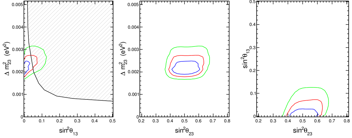
FIG. 7: Normal hierarchy contours for the SK-I+II+III data set. The 68%, 90%, and 99% allowed regions appear in blue, red, and green respectively. The shaded region in the first panel shows the Chooz 90% exclusion region.
