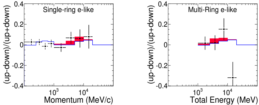
FIG. 11: Asymmetry (Up - Down)/(Up + Down) for the SK-I+II+III data set. Up is defined as events with \cos\Theta < -0.2 and down as \cos\Theta > 0.2 . Solid lines represent the MC expectation at the best fit from the \theta_{13} analysis and the shaded regions show the expectation at the best fit atmospheric variables but with \theta_{13} at the Chooz limit for the single- (multi-) ring e -like events at left(right). Error bars are statistical.
