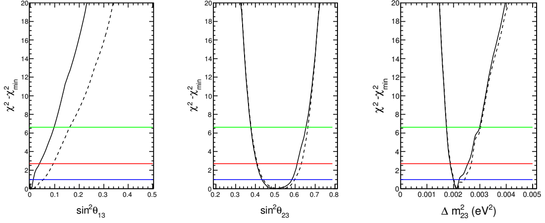
FIG. 9: The \Delta\chi^2 distributions for the SK-I+II+III data set in the normal (solid) and inverted (dashed) hierarchies. The horizontal lines represent the position of the one-dimensional cut value corresponding to the (from top to bottom) 99%, 90%, and 68% CL.
