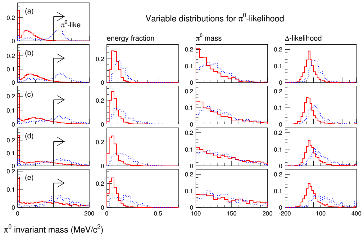
FIG. 3: The distributions used in the \pi^0 selection for five momentum regions: (a) P_e < 250 MeV/c, (b) 250 MeV/c \leq P_e < 400 MeV/c, (c) 400 MeV/c \leq P_e < 630 MeV/c, (d) 630 MeV/c \leq P_e < 1000 MeV/c and (e) 1000 MeV/c \leq P_e . Solid (dashed) lines represent CCQE (NC) events in the FC sub-GeV single-ring e -like Monte Carlo. Events with an invariant mass above 100 MeV/c 2 are selected as \pi^0 -like. To separate \pi^0 -like and electron-like more efficiently, an additional likelihood selection is applied for events with momentum above 250 MeV/c. The distributions of the three likelihood variables are shown: the fraction of energy carried by the second fitted ring ( E_2/(E_1 + E_2) ), the \pi^0 mass and \Delta -likelihood (described in the text). All distributions have been normalized to unit area.
