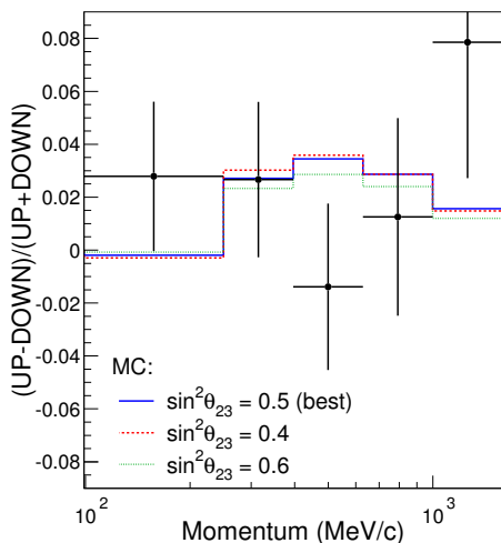
FIG. 6: Asymmetry (Up - Down)/(Up + Down) for the SK-I+II+III single-ring e -like 0-decay data set in the octant analysis. Up is defined as events with \cos\Theta < -0.2 and down as \cos\Theta > 0.2 . The solid line represents the MC expectation at the best fit point and the dashed (dotted) line shows the expected asymmetry for \sin^2\theta_{23} = 0.4(0.6) . The error bars are statistical.
